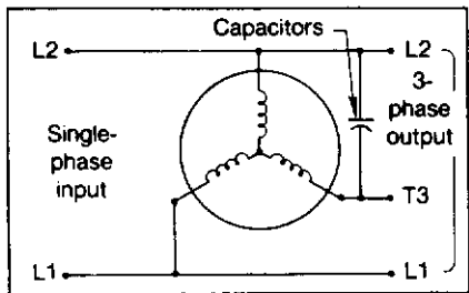
Figure 4 — Simplified equivalent circuit for a rotary converter.
