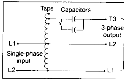
Figure 3—Simplified equivalent circuit for an autotransformer static converter.
