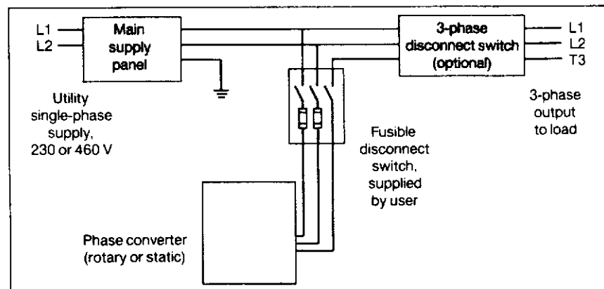
Figure 1 — Typical phase converter system.
